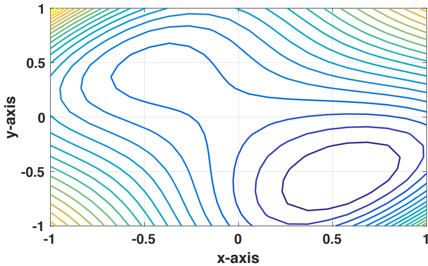
Figure 1: z = (x - y)^4 + 8xy - x + y + 3
