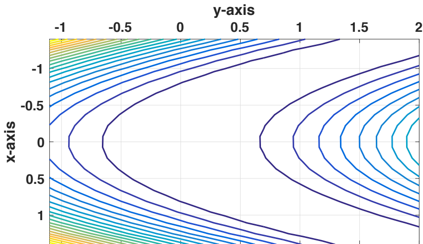
Figure 2: z = 100(x^2 - y)^2 + (x - 1)^2
